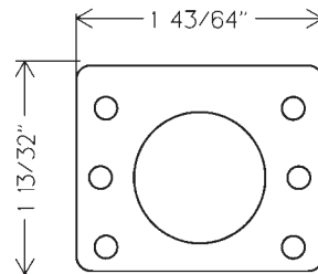
WP21 - 3/32 " spacer
