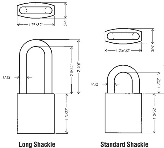
Long Shackle
